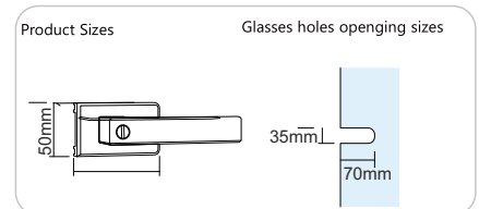
Cutout for CASP-MHL-06 & 10
